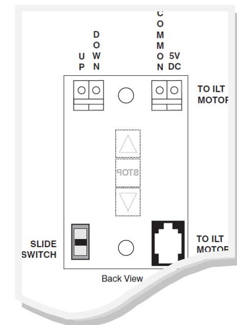
Back of ILT Wall Switch
